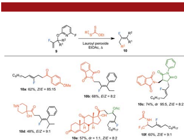
Figure 4. Scope of the radical olefination for vinyl fluorides. Reaction conditions: olefin (2 equiv), xanthate (1 equiv), lauroyl peroxide was added in 30 mol % portions (with respect to the xanthate) every hour (5–7 h). For 10c , the reaction was run in refluxing DCE.
