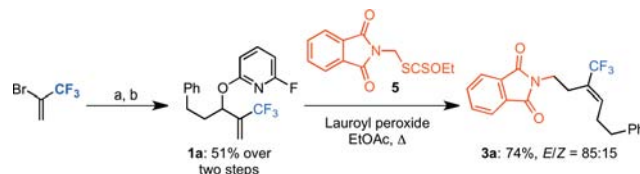
Scheme 2. Evaluation of Strategy A a
